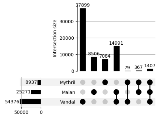
Figure 9: Overlap of bytecode tools detecting the suicidal vulnerability.
