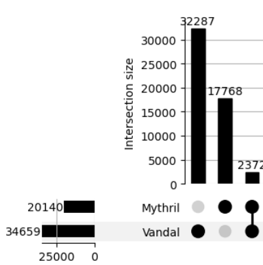
Figure 11: Overlap of bytecode tools detecting the txOrigin vulnerability.
