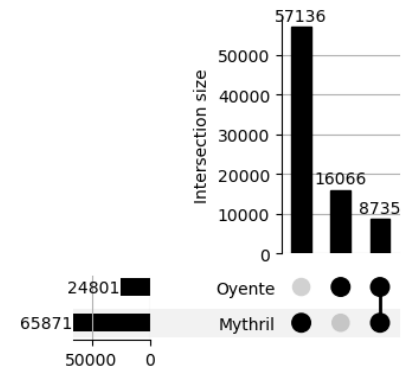
Figure 12: Overlap of bytecode tools detecting the Time Dependency vulnerability.
